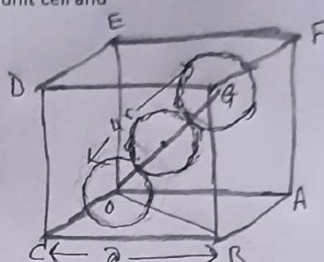
fig: Atoms in bcc unit cell
