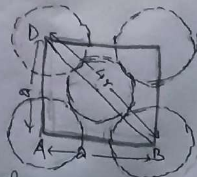
fig: Atoms in fcc unit cell.
